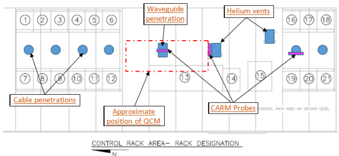
Figure 13, schematic layout of the electronics racks above Cave 1 showing approximate location of CARM probes on the Cave 1 rooftop. There is also a CARM in the Control Room.
