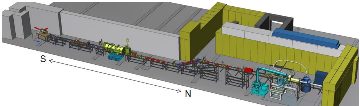
Figure 4: UITF layout showing the main exit towards the high bay area of the Test Lab and the MeV beamline and HDIce target. The MeV beamline is not relevant to this OSP but is shown for clarity.
