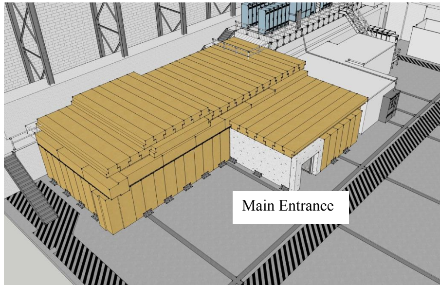
Figure 10: UITSF with concrete shielding in place
