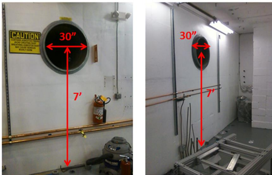
Figure 14: (Left) Fan with a capacity of 7400 CFM vents air into the high bay area, (Right) fan with a capacity of 4400 CFM vents air to outside the test lab
