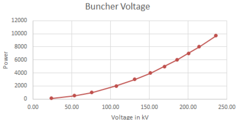
Figure 2: The possible acceleration capability of the normal-conducting copper-cavity 748.5 MHz buncher installed at UITF. When powered at 7 kW, a 200 keV input beam will gain 200 kV. This is considered a “worst case” scenario because it assumes electron beam parameters for the original FEL application (i.e., 500 kV input beam).
