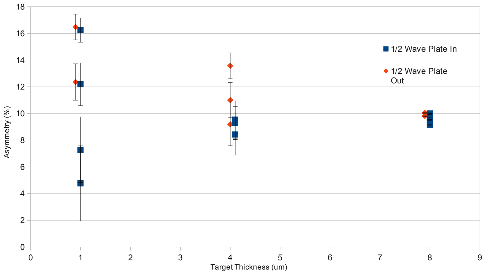
Copper : Asymmetry versus Target Thickness
