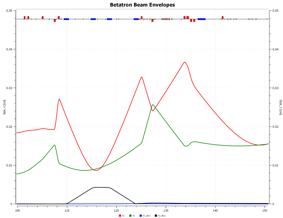
Figure 11. Beam envelopes of interim layout optimized for raster at pivot (right edge of plot). While the spot size is two-thirds larger than in figure 10, it is still below specification (0.03 cm, 300 microns). Colors as above.
