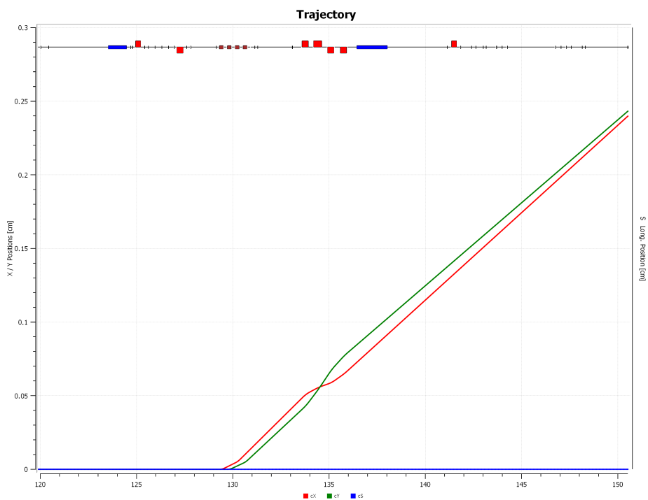
Figure 12. Raster with optics optimized for spot size at pivot, figure 10. Red horizontal, green vertical.
