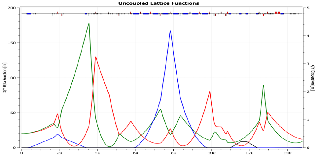
Figure 3. Beta functions (horizontal red, vertical green) and dispersion (horizontal blue, vertical black) throughout Hall A line to 32 cm past end of LH2 target. Dispersion uses right axis (m) and is peaked at the center of the arc leading to Hall A.
