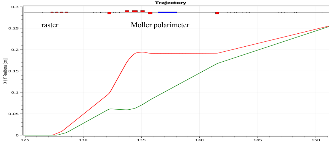
Figure 2. Raster response with subsequent quadrupoles set to provide envelopes in figure 1. 50 A horizontal (red) and 34 A vertical (green) drive. Note the horizontal scale change from figure 1; this figure shows only the last 26 m to the pivot vs 151 m there. X axis meters. Right axis unused.
