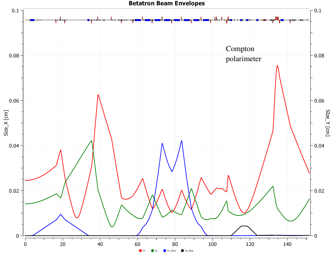
Figure 1. Normal target location is at the right edge of the plot. The horizontal beam size (red) is almost twice the vertical (green). This is a result of the competing constraints on the beam with inadequate variables. The blue line is the horizontal beam size due to dispersion with dp/p = 2E - 4 . The black line is the size due to vertical dispersion in the Compton polarimeter chicane. These need to be summed in quadrature with the red and green values, respectively. In the line at the top of all the images, red indicates quadrupoles and blue dipoles. X axis m.
