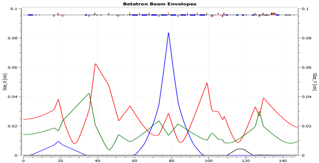
Figure 4. Beam envelopes, 1 mm full vertical scale, from start of Hall A transport line through to 32 cm past end of LH2 target. Color code as above. Horizontal (red) minima at right are at Compton polarimeter interaction point and at center of MOLLER LH2 target. Horizontal emittance is three times vertical so more focusing is needed. The quadrupole triplet, elements 241, 251 and 265, may be relaxed to move the final minimum either to the pivot or to \sim 4 m beyond it. Beam size would still be within agreed specification when relaxed to the latter extent. Blue line is envelope due to 4 m dispersion coupled to 2E - 4 momentum spread; horizontal position at the 1C12 BPM, at the peak, is dominated by energy changes (figure 3) just as beam envelope is.
