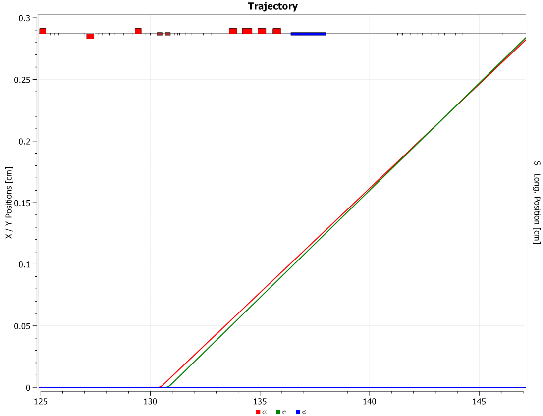
Figure 6. Raster response for MOLLER optics of section 7 is linear as all magnets after the raster are degaussed during production running. 74 A in vertical coil, green, for 5 mm square at center of target; 80 A for 5 mm square at upstream end of target chamber.
