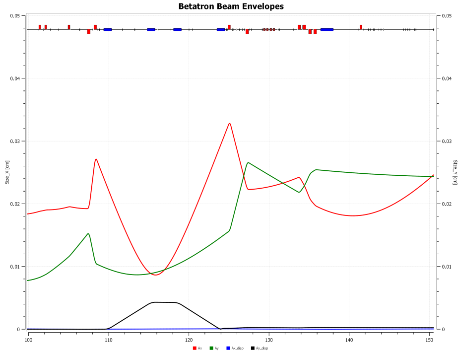
Figure 10. Beam envelopes of interim layout optimized for spot size at pivot (right edge of plot). Again, red horizontal and green vertical. Black: effect of vertical dispersion in Compton chicane.
