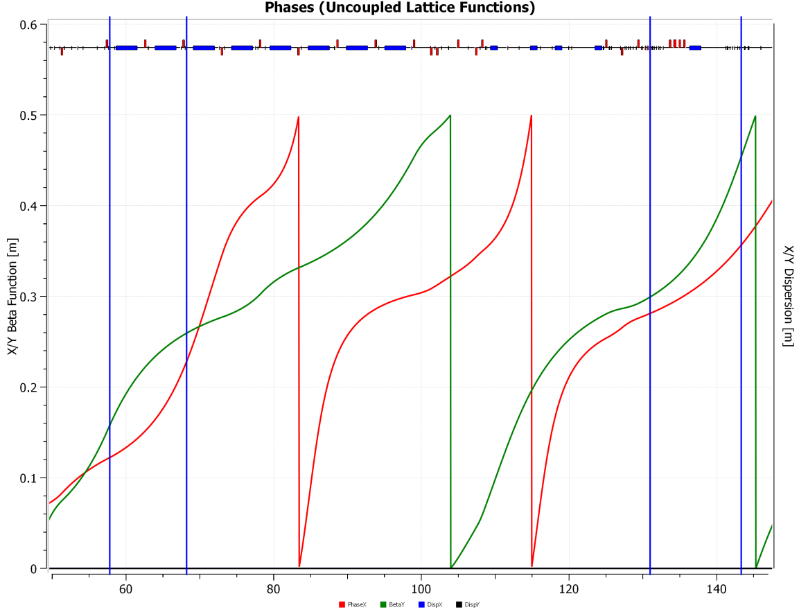
Figure 5. Phase advance from 1C07 quad to 32 cm past end of LH2 target. Color code as above: red horizontal, green vertical. The two vertical lines at left indicate the position of H/V coils which can be used to excite small position variations to quantify helicity dependent position differences. The two lines at the right are BPMs after all excited magnets. There is adequate but not optimal phase difference between the exciting coils and the BPMs. There are two intermediate BPMs on the right not indicated. The four BPMs in question are elements 275, 287, 301 and 321. Two cavity BPMs are also in this region. If the phase advance proves inadequate one of the coil pairs may be moved farther upstream during or after the first sixteen week MOLLER run.
