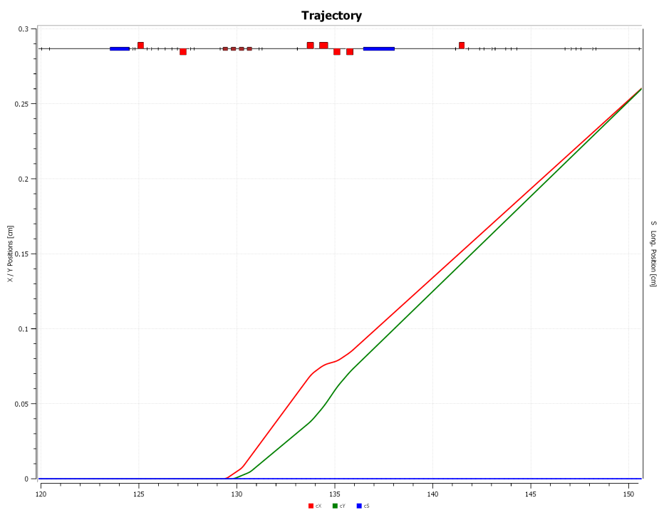
Figure 13. Raster with optics optimized for near-equal coil currents, so a circular raster would be easy to implement. Envelopes in figure 11. Colors as above.
