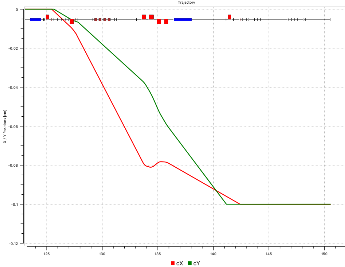
Figure 9. Correction of 1 mm target offsets in both X (red) and Y (green) in the interim optics solution.
