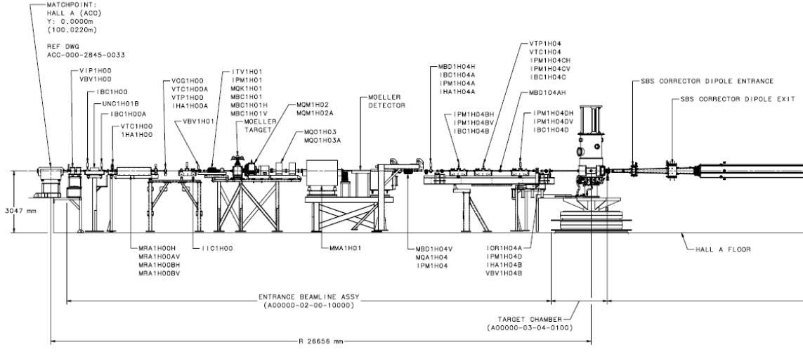
Figure 14. Existing beam line.
