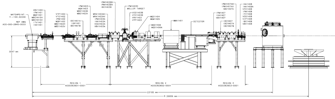
Figure 15. MOLLER beam line.
