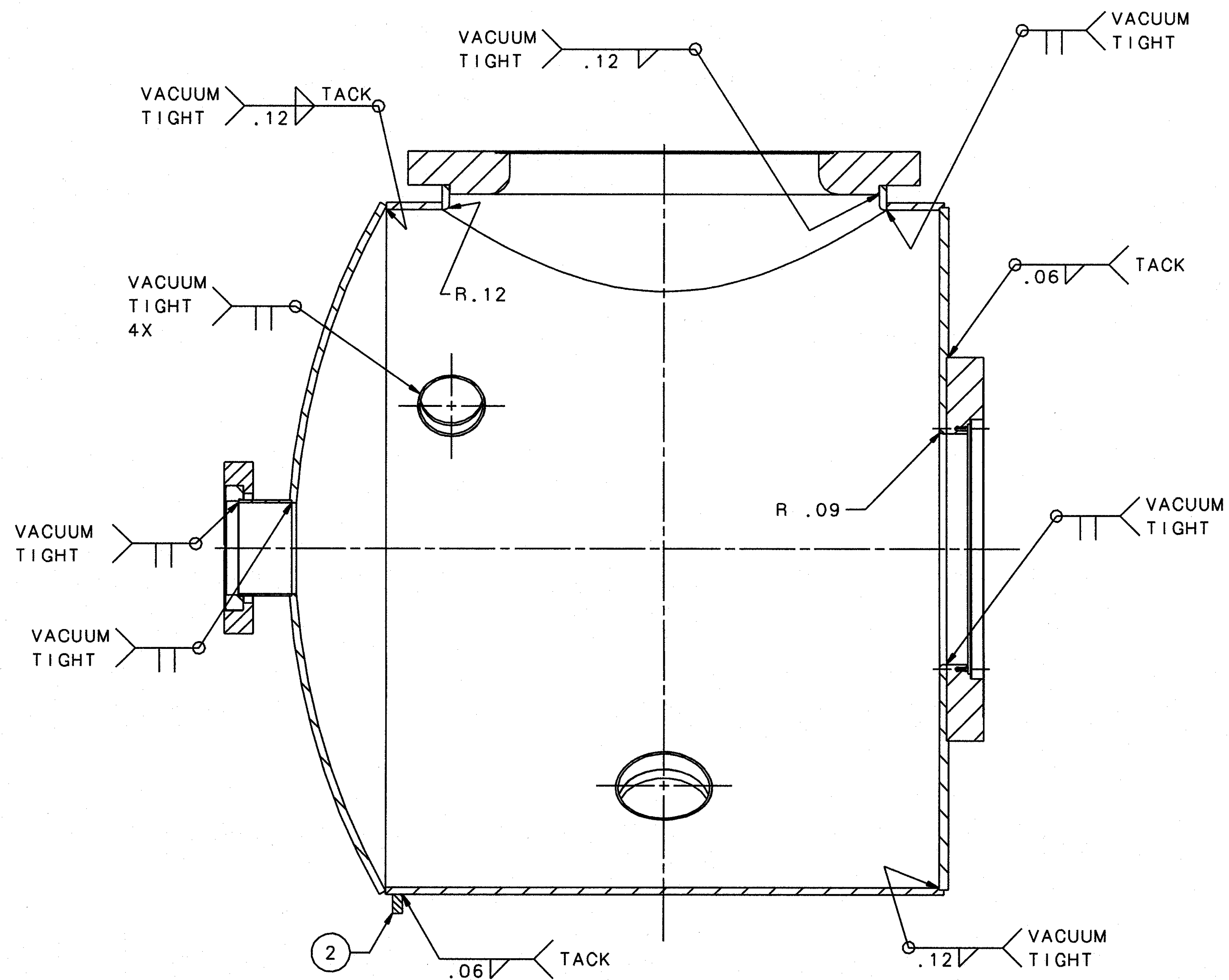
SECTION B-B
