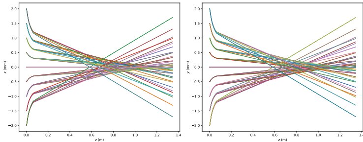
← Figure 4: Particle trajectories started on a 2 mm \times 2 mm grid in the R28 gun, POISSON model.
