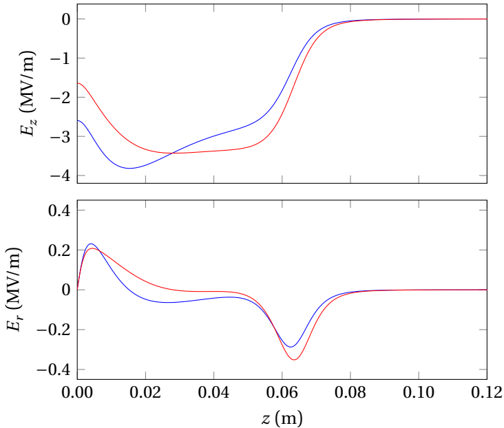
← Figure 3: Axial (top) and radial (bottom, at x = 3 mm) electric field in the R28 and R30 guns simulated with Poisson.
