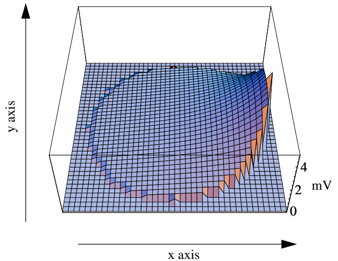
Figure 3: Typical two dimensional map of a BPM lobe response. Center is at x = 0, y = 0 and grid squares are 0.5 mm on a side. The z axis is the lobe signal for a given wire position in mV.
