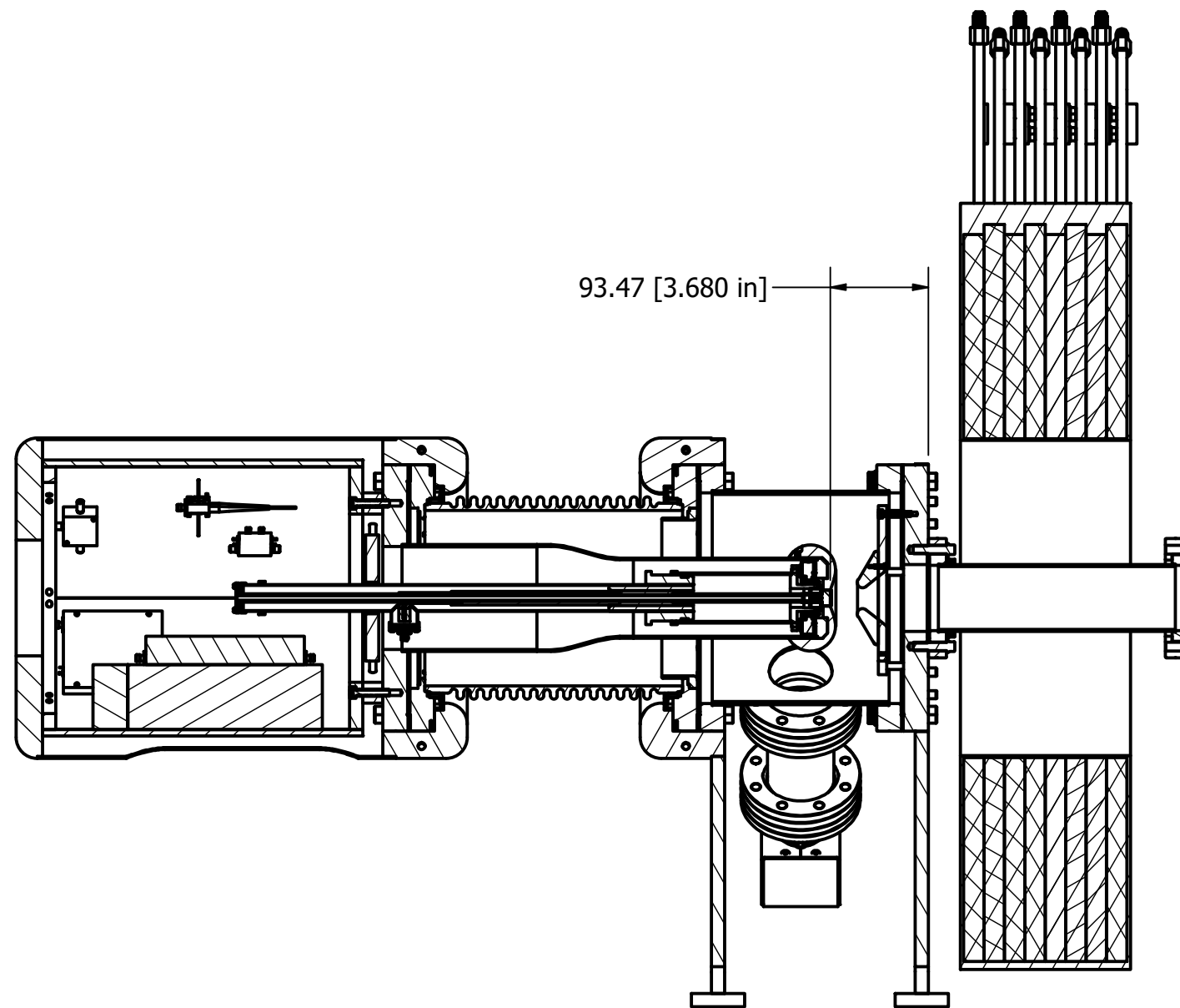
SECTION A-A SCALE 1 / 6
