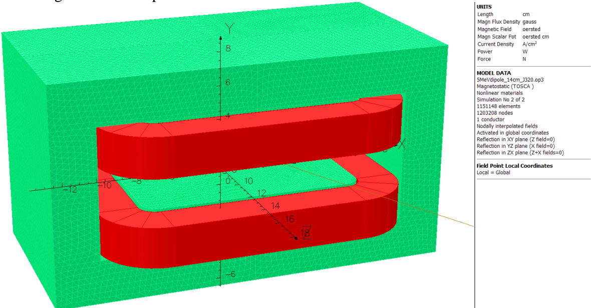
Figure 2. Proposed 5 MeV dipole 14 cm wide poles vs 4", 12.5 cm long vs 4"
