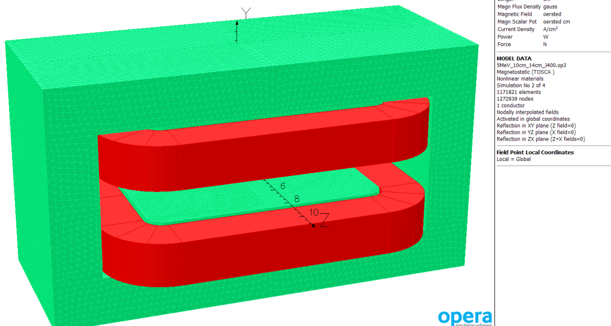
Figure 8. 14 cm wide by 10 cm long pole with 1 cm radius on corners. 1010 steel BH curve used.
