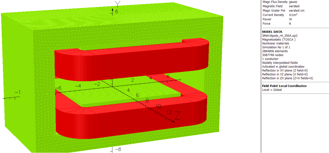
Figure 1. Original 5 MeV dipole
