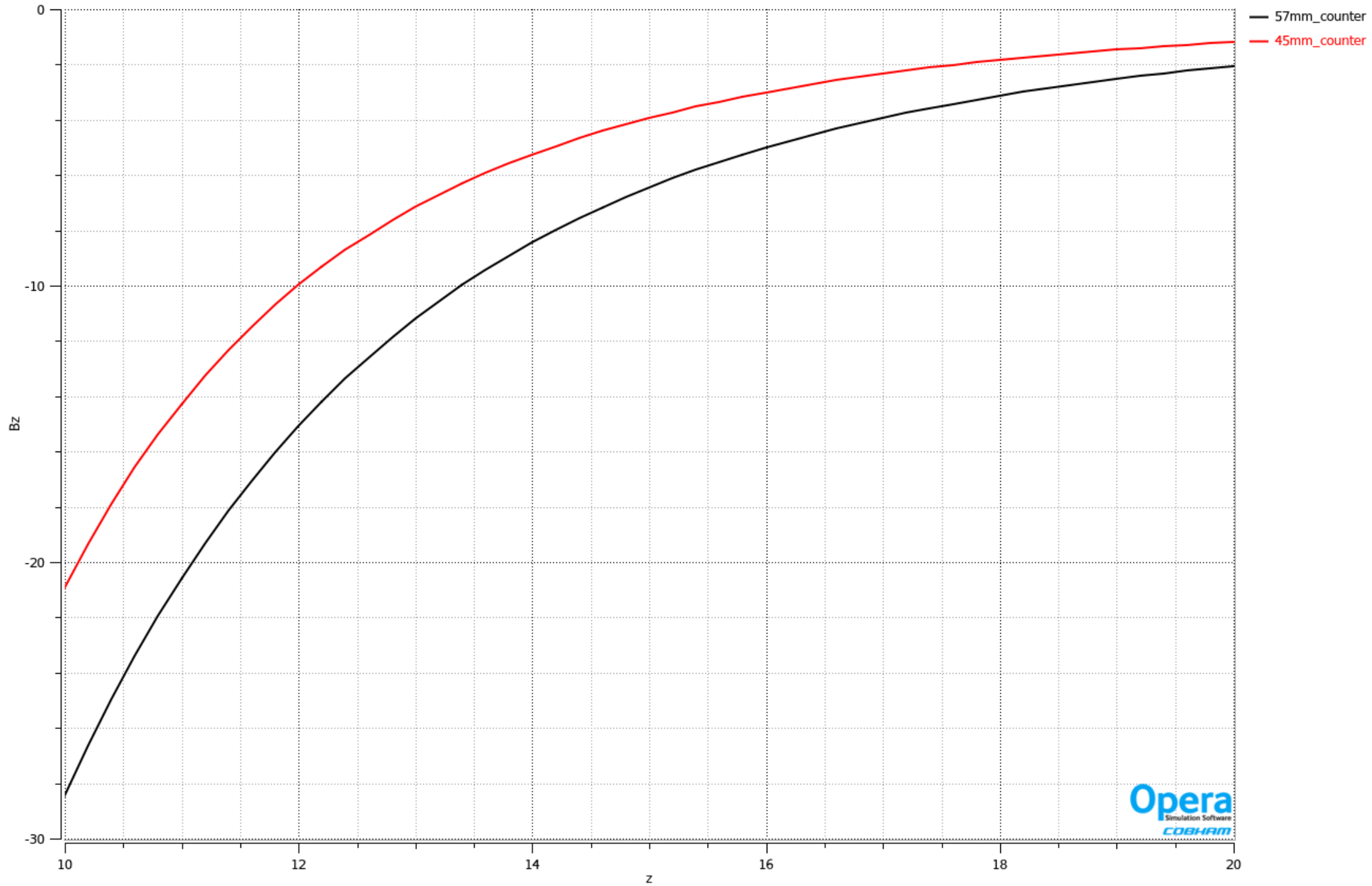
stray field counter-wound vs steel radius
