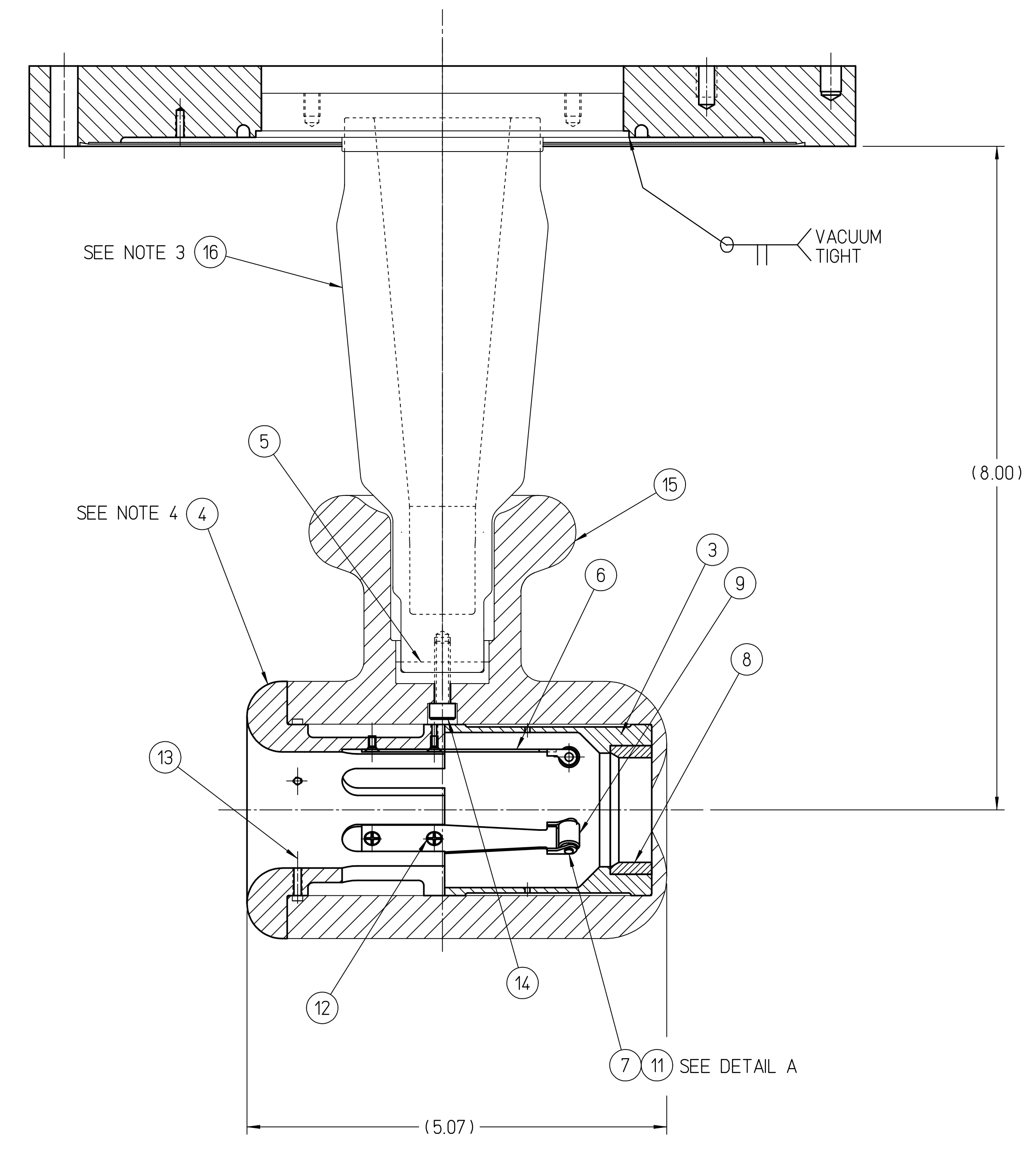
ASSEMBLY -02
