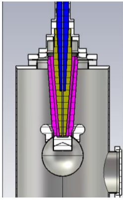
Fig. 2. SolidWorks model showing a cross section of the high voltage testing apparatus. Blue: Vulcanized rubber high voltage cable termination. Gold: Modified commercial epoxy receptacle. Pink: 500 kV doped alumina inverted insulator. The spherical electrode is 0.2 m diameter.
