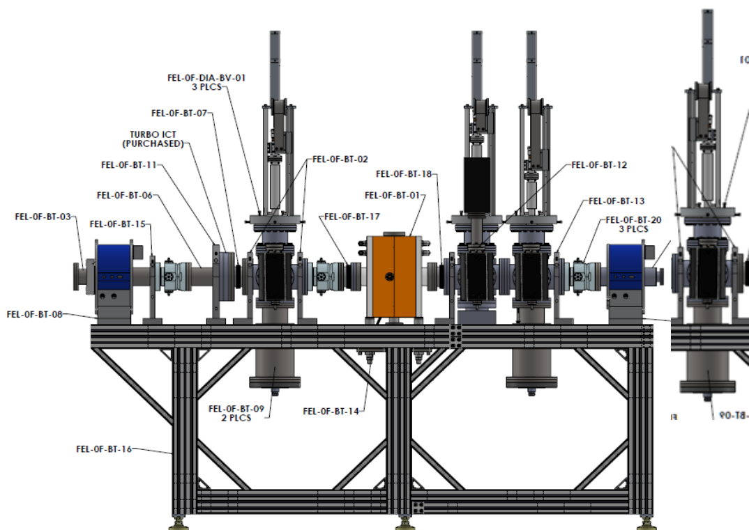
Figure 5: The existing beamline between the gun and the dump. This beamline will be modified to install the three skew quadrupoles. The buncher will not be installed (orange object)
