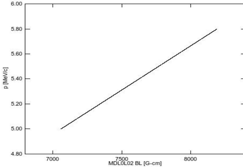
Fig. 2. TOSCA prediction of momenta vs. straight field integral for +25.0° deflection.
