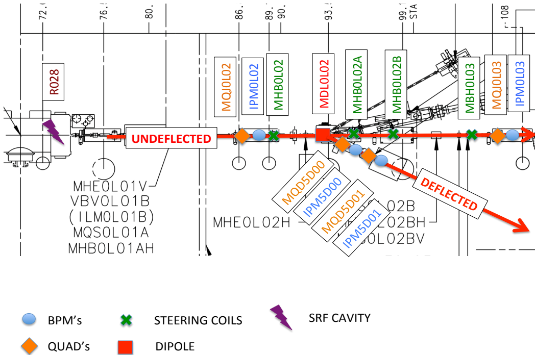
Fig. 1. Picture shows the layout and names of the relevant beam line elements.
