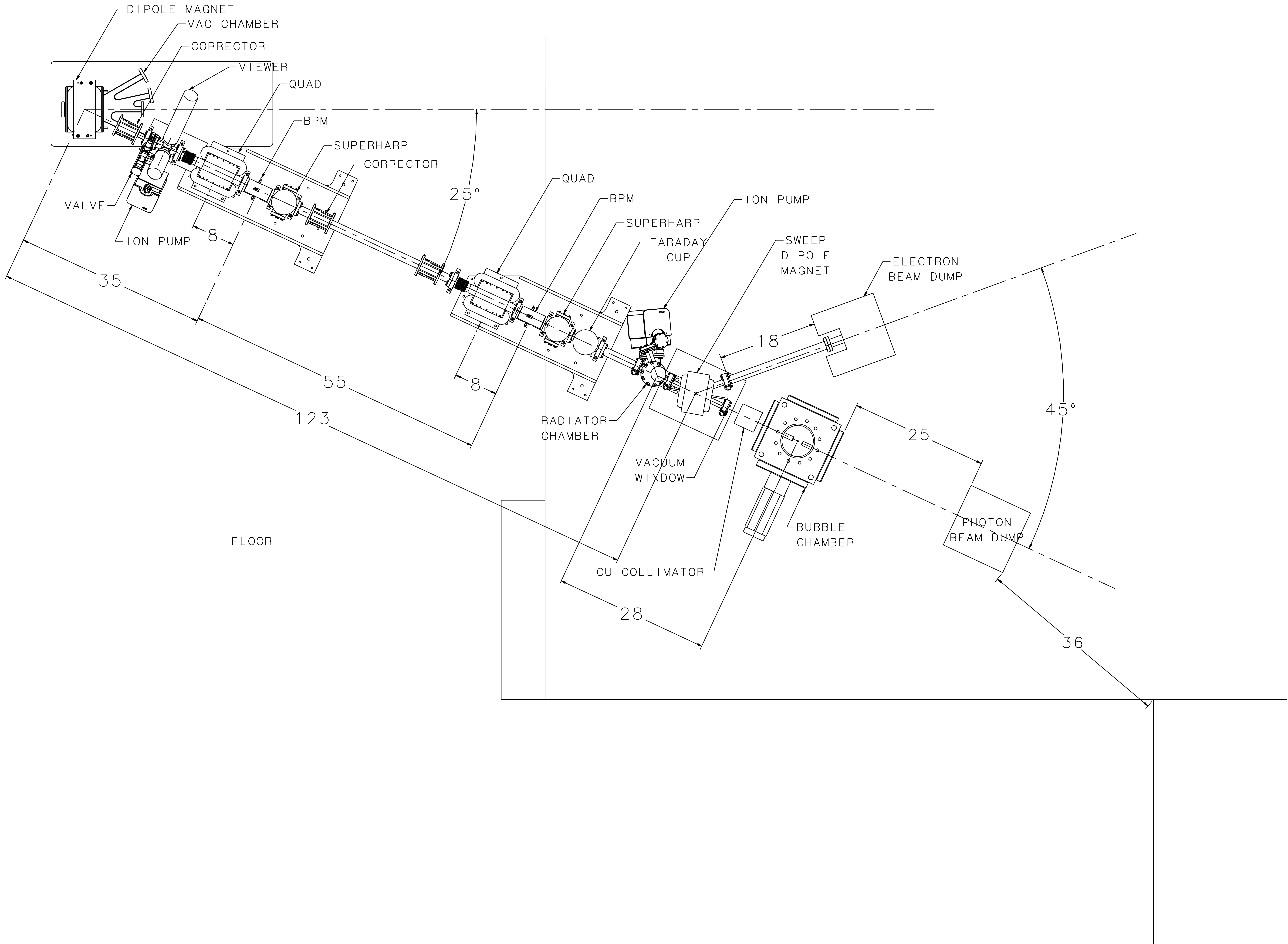
VIEW A
