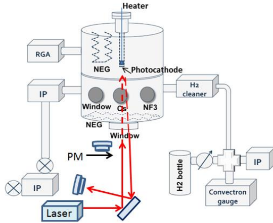
Figure 3: Schematic of the vacuum test chamber used to measure QE versus laser wavelength. IP: ion pump, NEG: non-evaopable getter pump, PM: laser power meter. A schematic of the low voltage Mott polarimeter can be found in reference [5].
