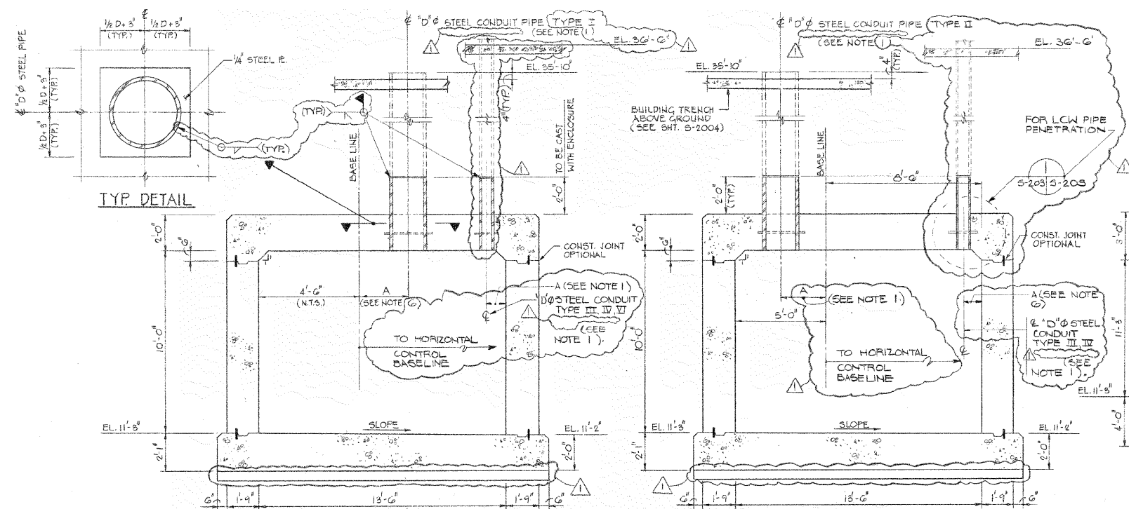
ACCELERATOR ORIGINAL CONSTRUCTION (AS-BUILTS) - TYPICAL TUNNEL SECTION
