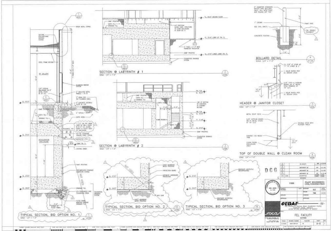
LERF ORIGINAL CONSTRUCTION (AS-BUILTS) - LABYRINTH SECTIONS
