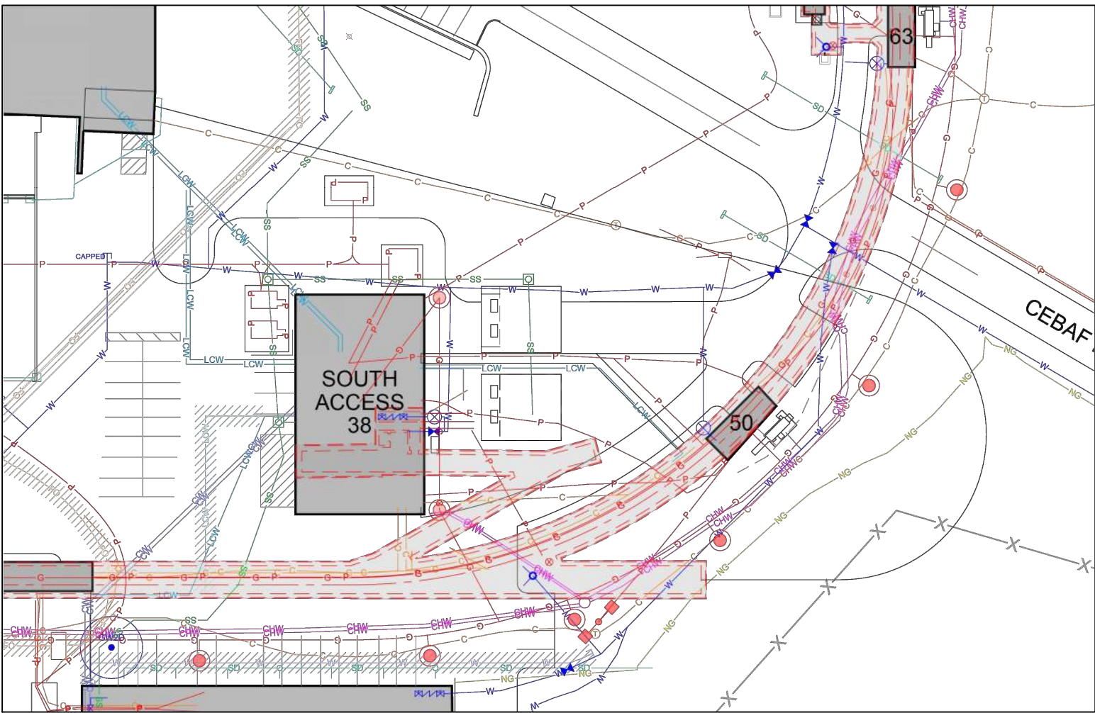
UTILITY INTERFERENCE - SITE PLAN
