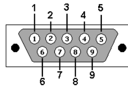
9 Pin Male D
