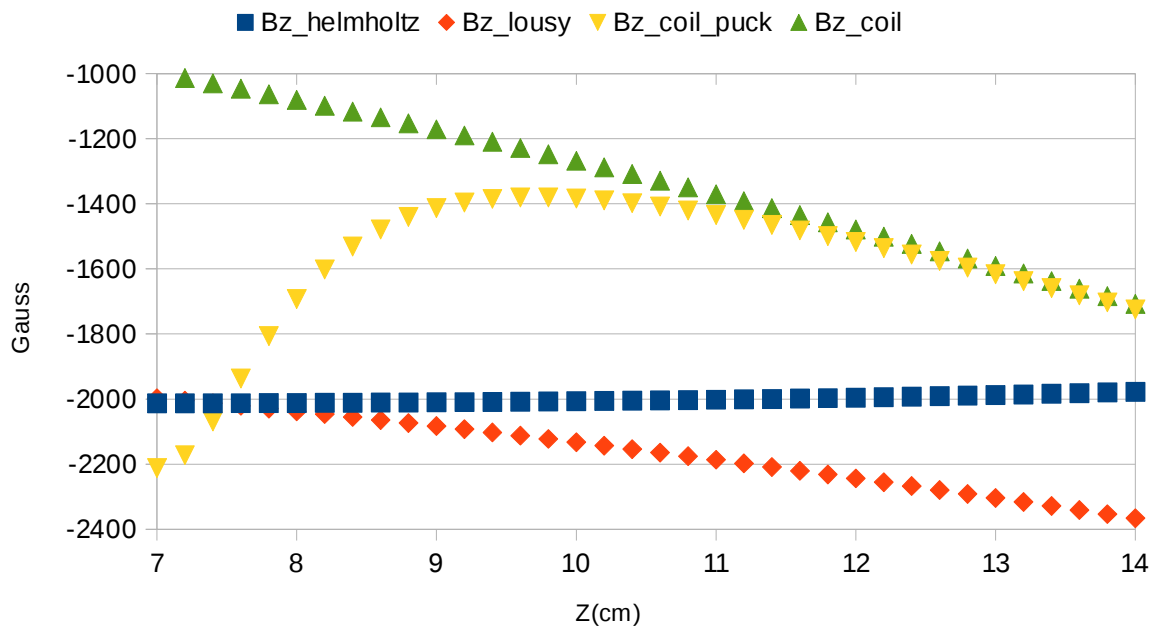
Figure 18. Bz for four models from near cathode (7.5 cm) to anode
