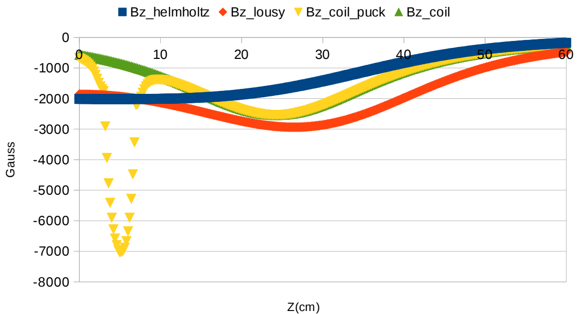
Figure 17. Bz for four models over the 60 cm with relatively fine mesh Bz(60) for the four models: -174.6, -471.5, -247.2, -247.2. First and second have shields, third and fourth don't.
