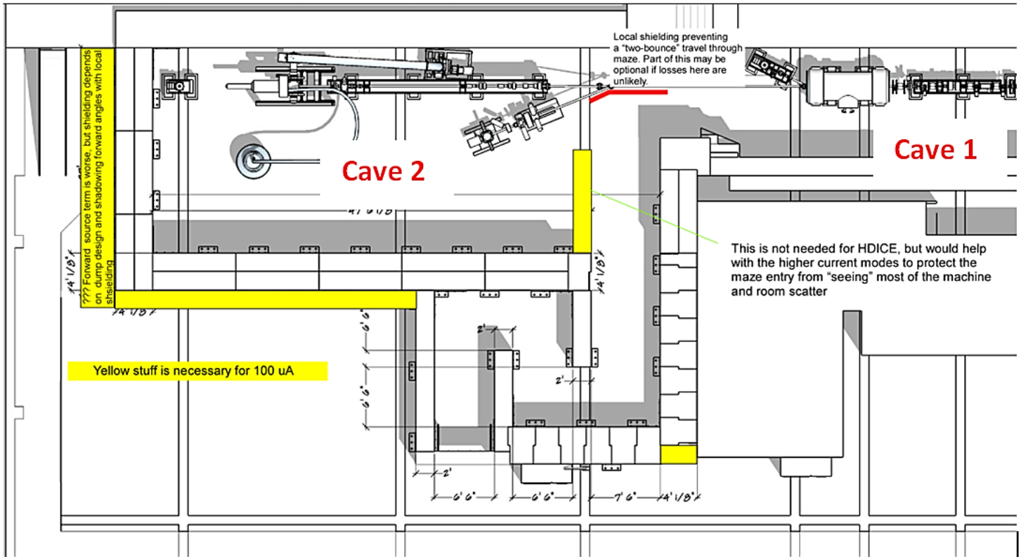
Figure 1 UITF beamline layout showing the two Caves. keV beam is confined to Cave 1
