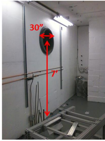
Figure 8 (Left) Fan with a capacity of 7400 CFM vents air into the high bay area, (middle) fan with a capacity of 4400 CFM vents air to outside the test lab, right two chimneys attached to the square vent holes in the ceiling of Cave 1
