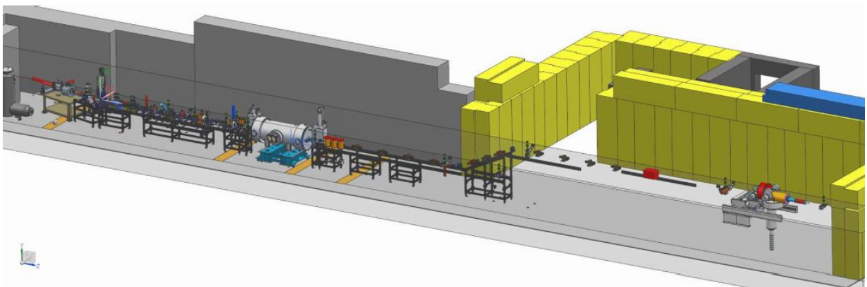
Figure 2 UITF layout showing the exit to main entrance through labyrinth towards the high bay area
