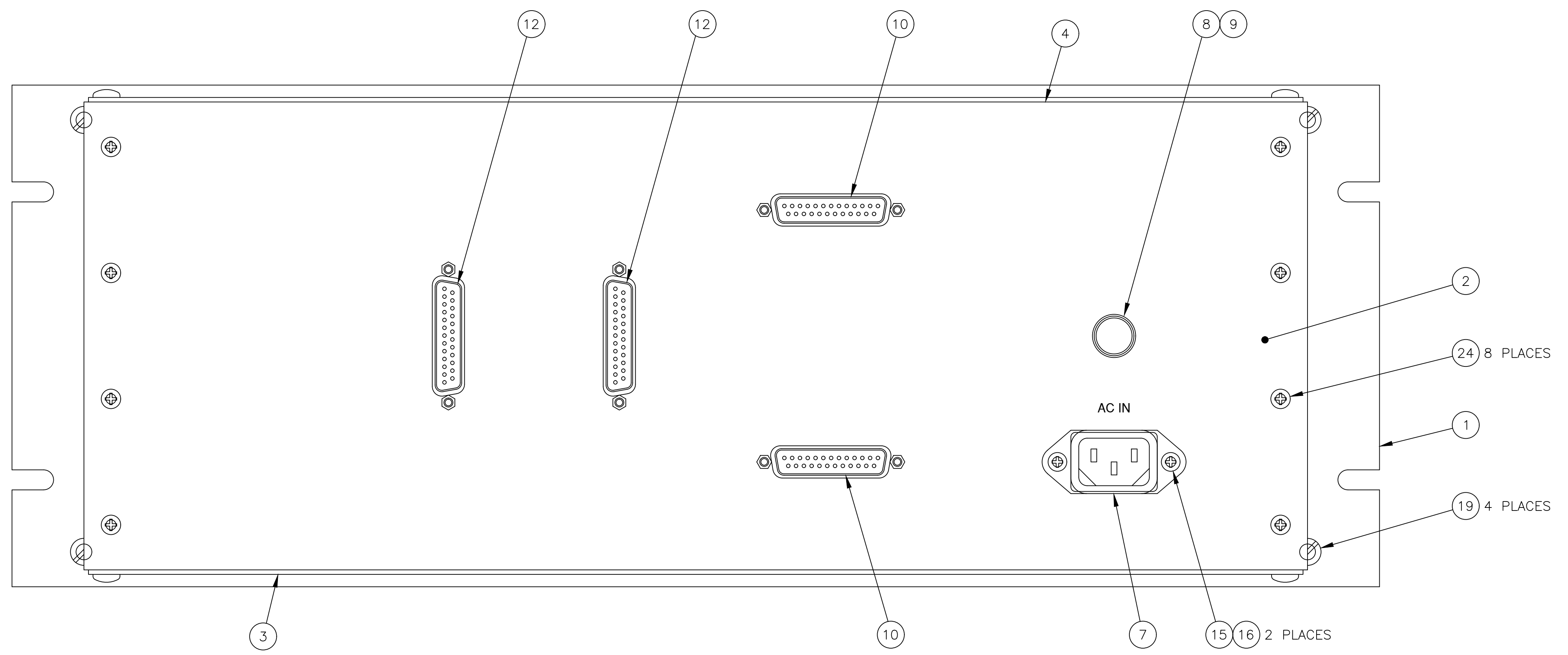
VIEW B-B
