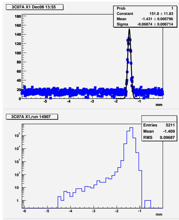
Figure 4: Scan of 3C07A superharp X wire. The upper panel shows the superharp response with current readout. The lower panel shows the response of a high rate PMT. Note the halo tail observed with the PMT readout.
