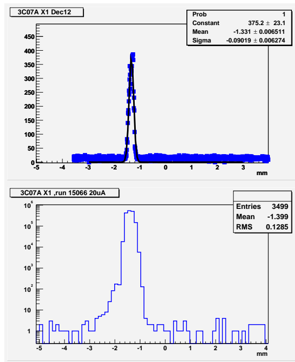
Figure 5: The same as Figure 4, but with a reduced halo tail.
