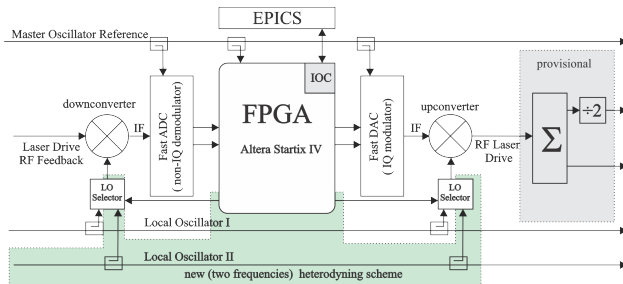
Figure 2: Architecture of the LLRF hardware for an individual laser. Signal processing involves mixing with the Local Oscillator to down and up convert RF signals, digital demodulation, Proportional-Integral control, and generating the Intermediate Frequency (IF) signal using a single Digital to Analogue Converter (DAC) [8]. The clocks for the FPGA and Fast ADC/DAC are derived from the Master Oscillator Reference. The Local Oscillators for the up and down conversions are coupled from the Local Oscillator lines. The green area shows the proposed addition to the LLRF to allow system operation at two frequencies while the grey is the present configuration.
