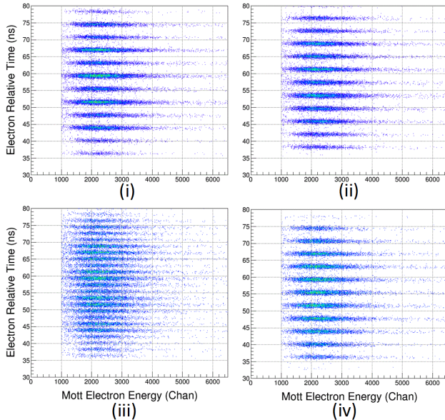
Figure 4: Timing of 250 MHz beam bunches measured in Mott polarimeter (i) Beam A only, (ii) Beam D only (note bunches shifted in time by 2 ns), (iii) A+D 2 ns apart, (iv) A+D 0 ns apart after D timing changed to match A.
