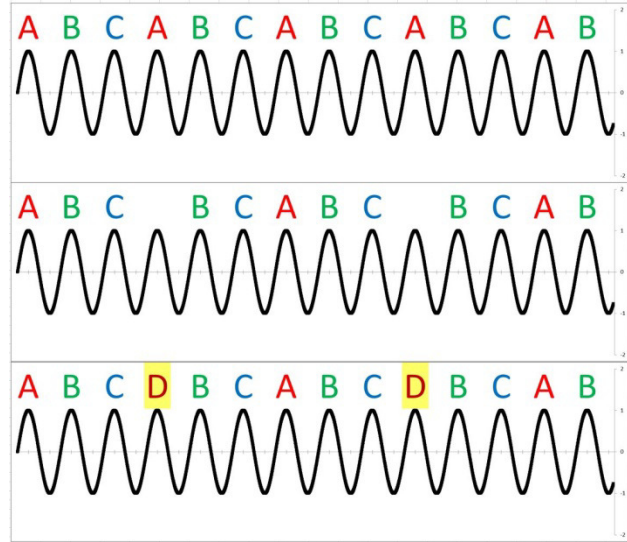
Figure 1: Each sine wave represents the 1500 MHz accelerating frequency. Top, three interleaved beams (A, B, and C) each at 500 MHz. Center, A beam at 250 MHz makes room for D beam. Bottom, A and D at 250 MHz and B and C at 500 MHz.
