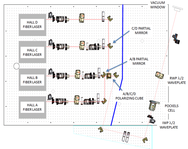
Figure 5: The 4-laser configuration. Once the four laser beams are combined, all four traverse the same Pockels cell and waveplates which are used to convert the linearly polarized lasers into circularly polarized lasers prior to reaching the entrance window to the electron gun vacuum system.
