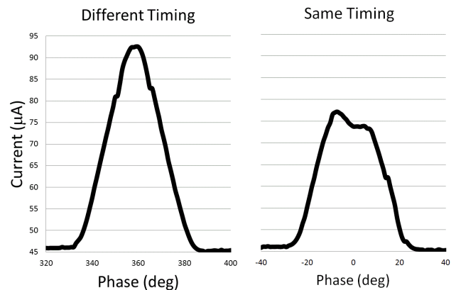
Figure 3: Total current from two 250 MHz beams each at 45 \mu\text{A} peak. Left: the beams are 2 ns apart in time. Right: the two beams have simultaneous pulses showing signs of higher space charge.
