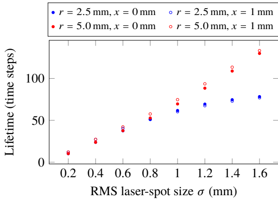
Figure 4: Lifetime as a function of laser-spot size for active areas of different radii r and different horizontal laser-spot displacements x .
