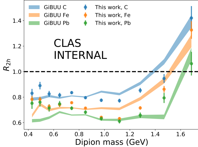
Figure 3. CLAS6 Preliminary result : Conditional suppression factor as a function of pion pair invariant mass. Points are slightly shifted horizontally for visibility. The error bars in the CLAS data represent statistical uncertainties only. No acceptance or radiative-effect correction has been applied.
