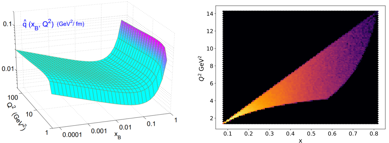
Figure 1. Left: Transport parameter coefficient \hat{q} extracted by Ru et al. [27] from a global fit to SIDIS, Drell-Yan and quarkonia production in proton-nucleus collisions. Right: Kinematic coverage for 11 GeV beam subject to CLAS12 acceptance, and the following selection: W > 2 GeV and y < 0.85 and at least one hadron with z > 0.4 .
