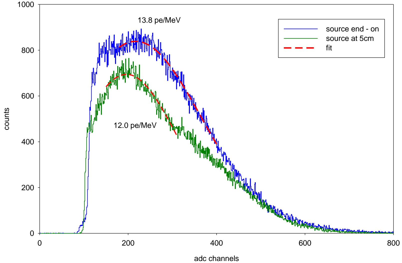
Light output - Crystal #15 - grease-coupled pmt, full coverage
