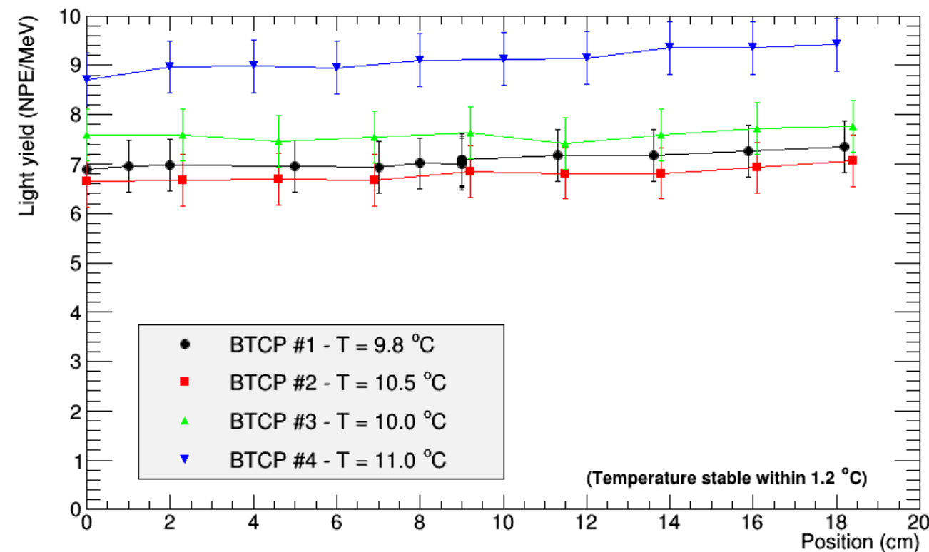
BTCP's crystals
