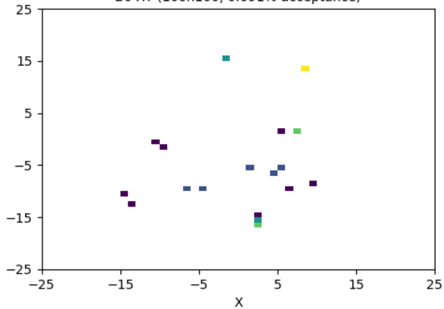
B0 XY (10on100, 0.091% acceptance)
