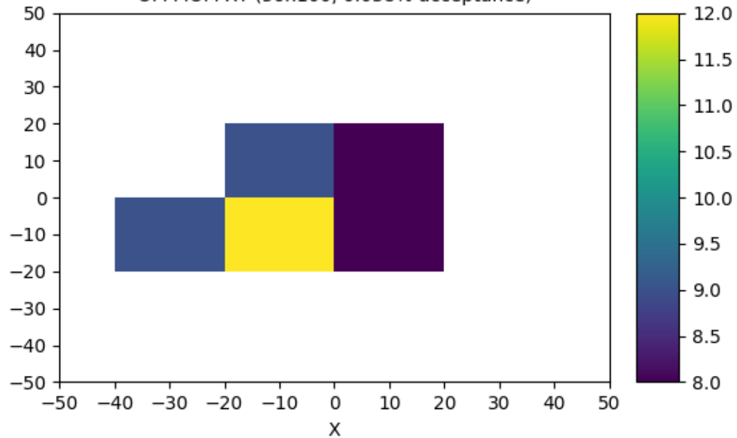
OFFMOM XY (18on275, 0.034% acceptance)
