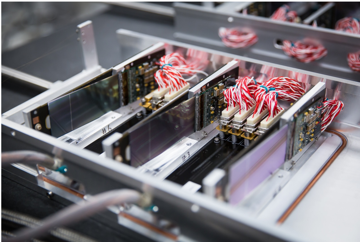
FIG. 7: A photograph of the u-channel support structure that holds the Layer 1-3 modules of the SVT. Layer 0 would be mounted on this support in roughly to same position as the wire scanner support seen at left, with scan wires moved slightly upstream towards the target. The crossover boards that provide power and readout for the modules can be seen between the SVT modules, where the two unused connections on the crossover board between layers 1 and 2 can be used for Layer 0.
