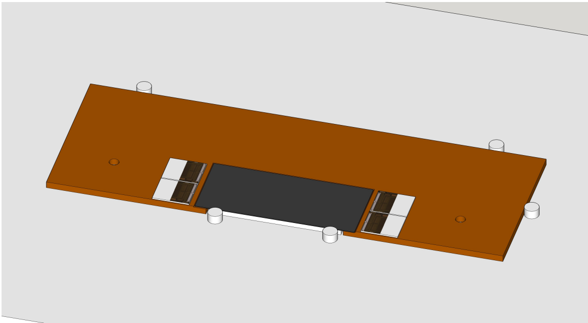
FIG. 9: The conceptual design of the Layer 0 hybrids. The sensor is mounted on the step in the window of the hybrid.
