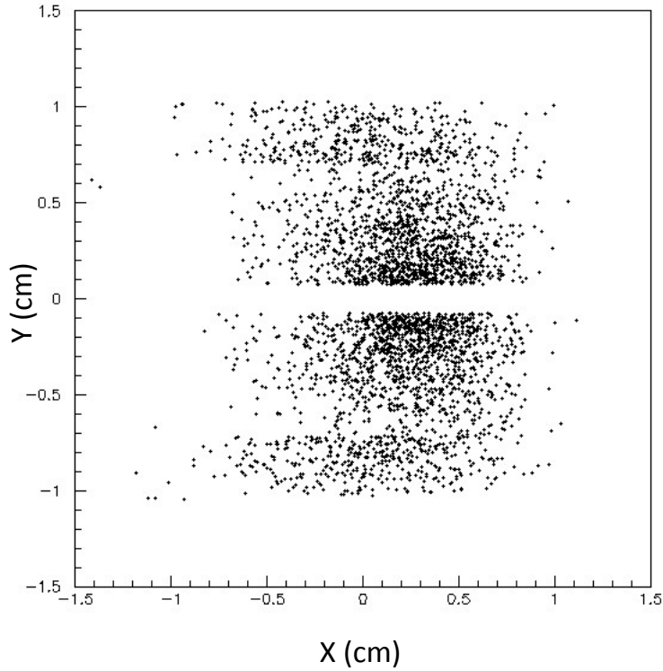
FIG. 6: The distribution of hits from electron recoils that also produce hits in Layers 1 and 2. Together with the beamspot constraint, such recoils can be reconstructed with high efficiency. Including the recoil in a kinematic fit significantly increases the sensitivity of the resonance search.
