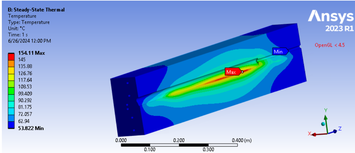
Fig. 1 CPS Copper Absorber Temperature Distribution – section cut down the middle
