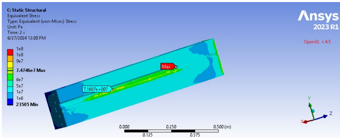
Fig. 2 CPS Copper Absorber Thermal Stresses
