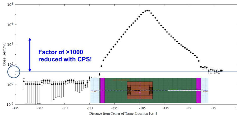
Fig. 12. Prompt radiation dose rate as a function of upstream distance from the target for the case of a 2.7 \mu A electron beam hitting a 10% copper radiator inside the CPS. The dose includes contributions from all particles. The large reduction factor of >1000 as a result of the CPS shielding is apparent.
