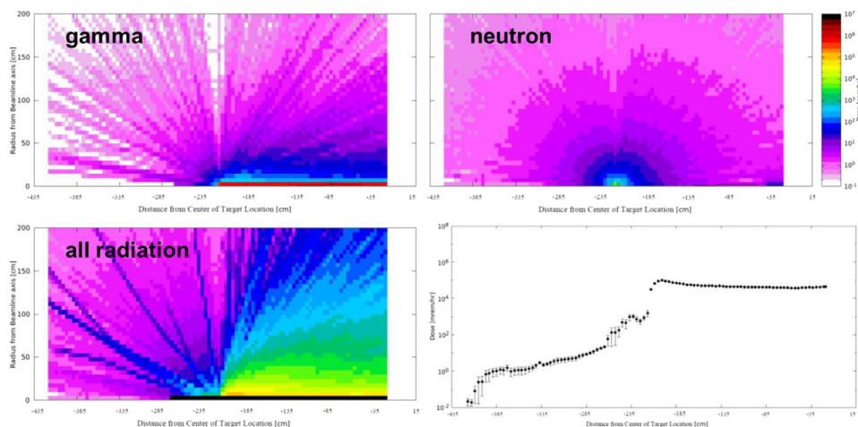
Fig. 11. Prompt radiation dose rate as a function of position in the experimental hall for the case of a 2.7 \mu A electron beam hitting a 10% copper radiator. Two-dimensional plots are shown for the dose from photons only (top left), from neutrons only (top right) and from all particle types (bottom left). Also shown is a one-dimensional plot of prompt dose rate along the beam direction (bottom right).
