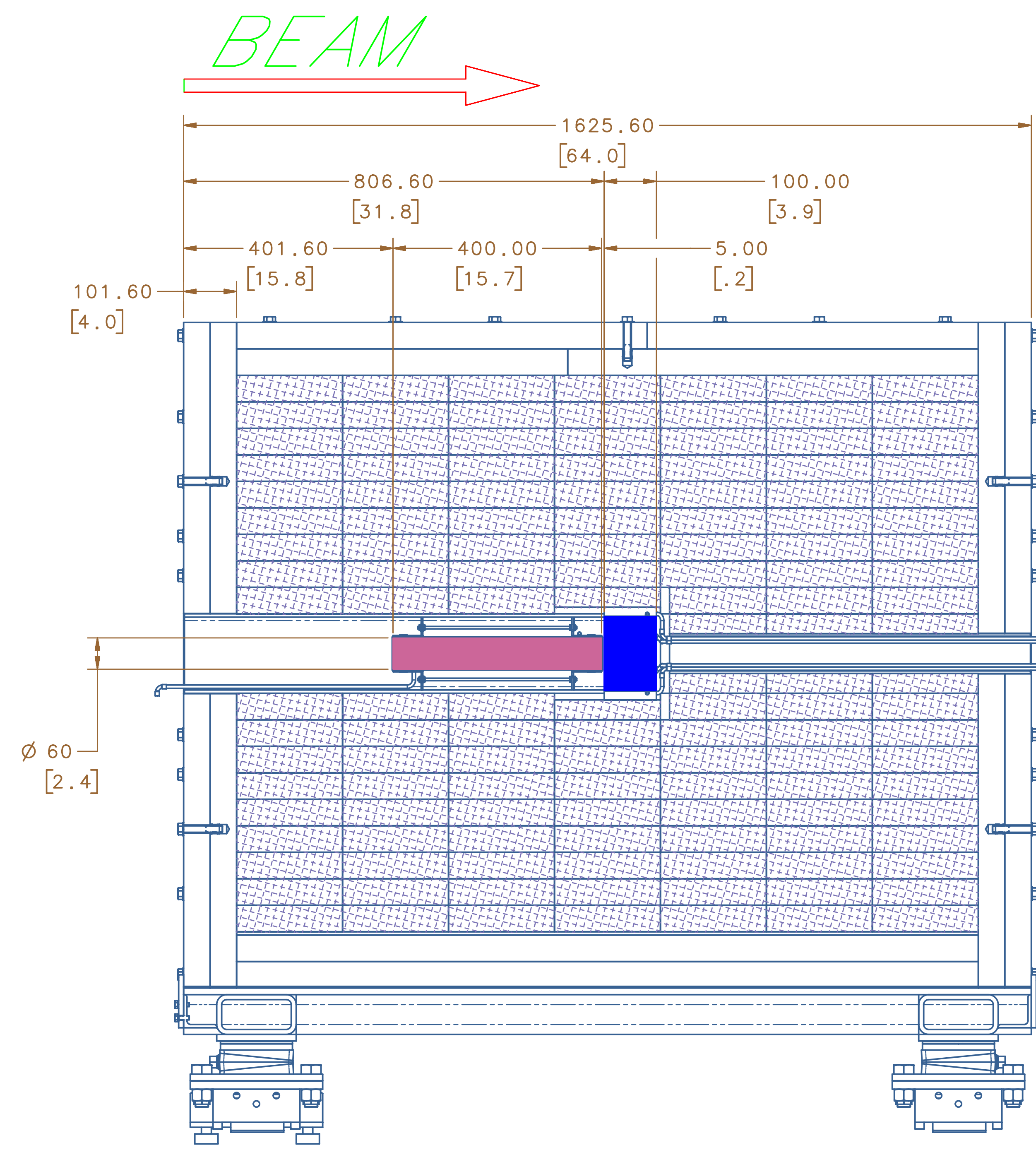
SECTION B-B
