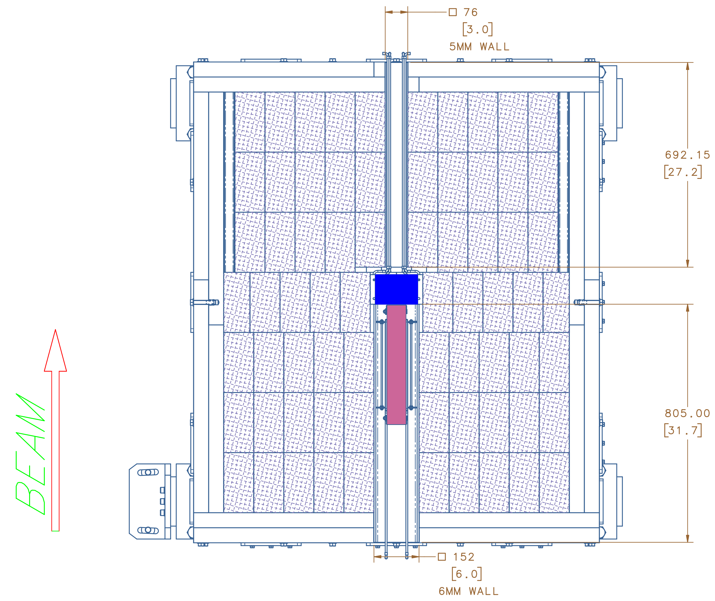
SECTION C-C
