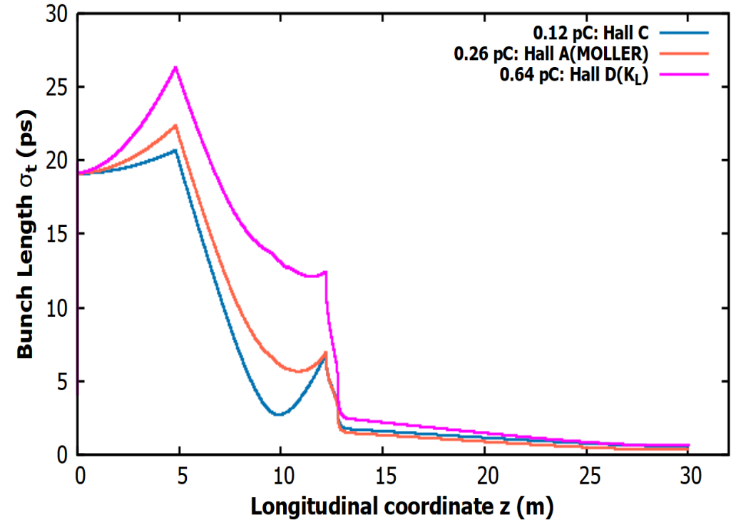
Evolution of bunch length along the beamline for various charges per bunch.
