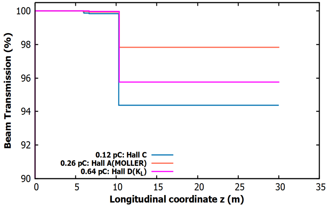
Transmission for various bunch charge specifications for the CEBAF four halls.
