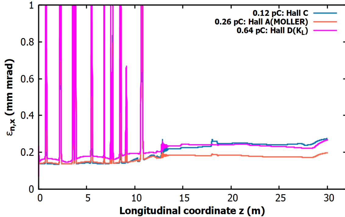
Transverse horizontal and vertical normalized emittances for different bunch charges.
