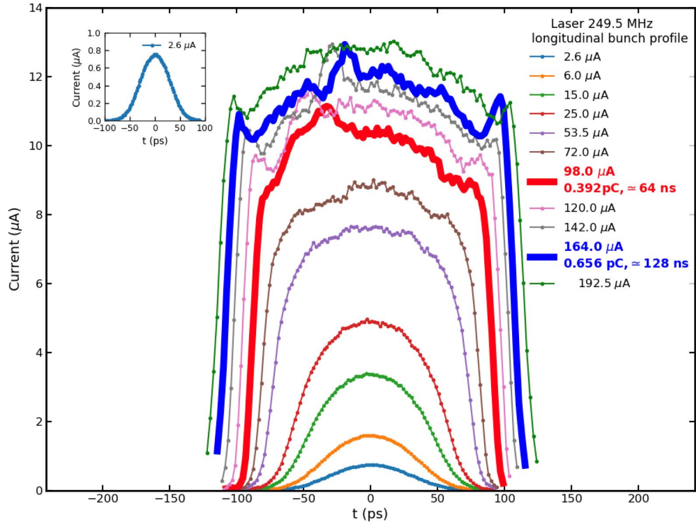
Electron Bunch-length measurements at 249.5 MHz laser at the location of chopper.
