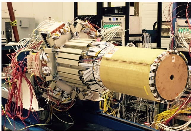
Fig. 28. The fully assembled Central Vertex Tracker with the SVT, BMT, and FMT. The BMT and FMT are shown on the outside. The FMT has a circular opening in the center for the electron beam to pass through. The SVT is encapsulated and hidden from view.
