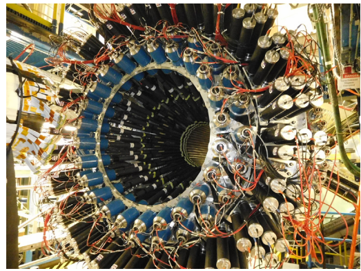
Fig. 30. The fully assembled CD as seen from its upstream end with the 144 CND light guides and PMTs at the three outermost rings, and the 48 PMTs of the CTOF (two inner rings).
