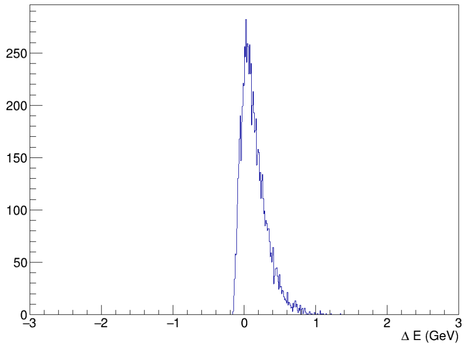
Figure 4: Beam Momenta p_{KLong} > 3.75 GeV
