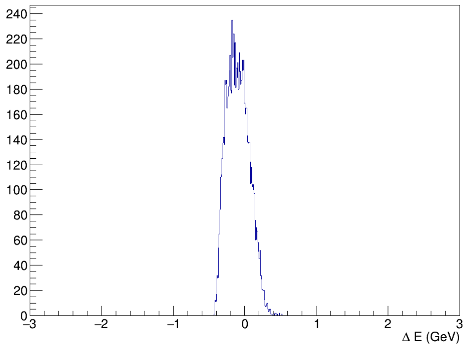
Figure 2: Beam Momenta 2.5 < p_{KLong} < 3.0 \text{ GeV}
