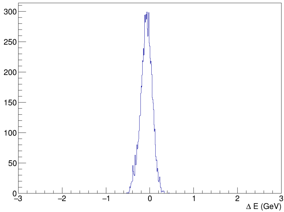
Figure 1: Beam Momenta p_{KLong} < 2.5 \text{ GeV}
