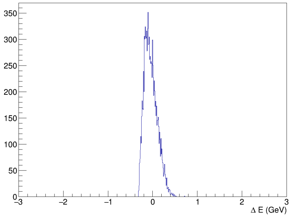
Figure 3: Beam Momenta 3.0 < p_{KLong} < 3.75 GeV
