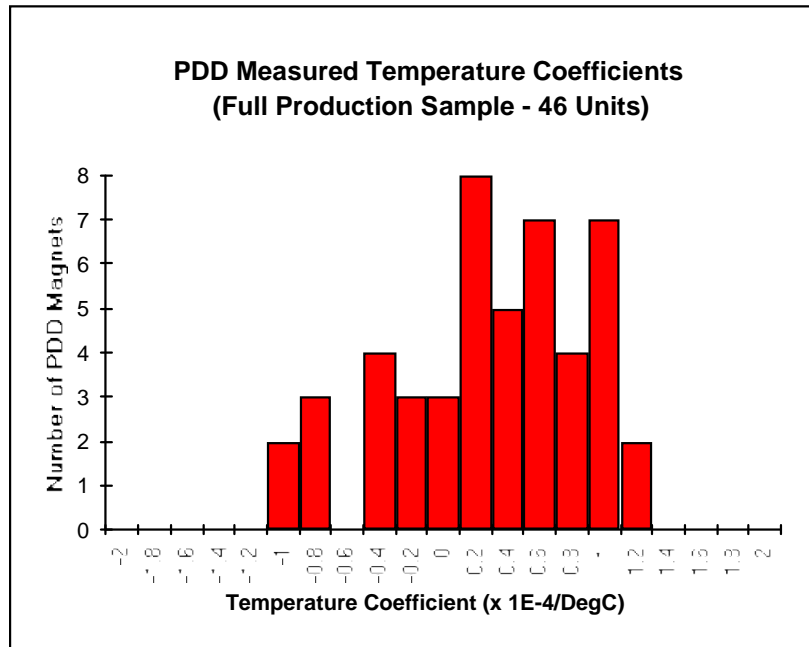
Figure 3.1A-10. Temperature Coefficients measured for the production run of PDD magnets. The mean is 0.15 units/ ^{\circ}\text{C} , the standard deviation is 0.60 units/ ^{\circ}\text{C} , and the acceptance tolerance was 1.2 units/ ^{\circ}\text{C} .
