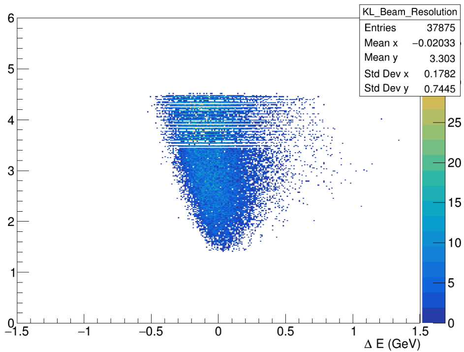
Figure 2: Beam Resolution
