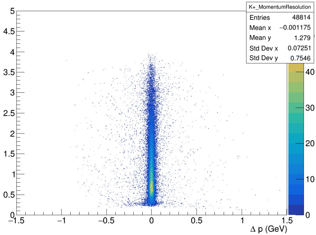
Figure 3: K^+ Resolution
