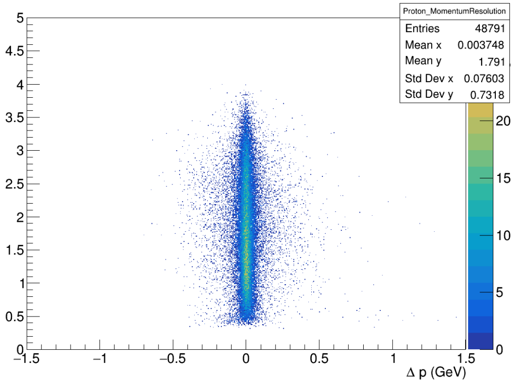
Figure 4: Proton Resolution
