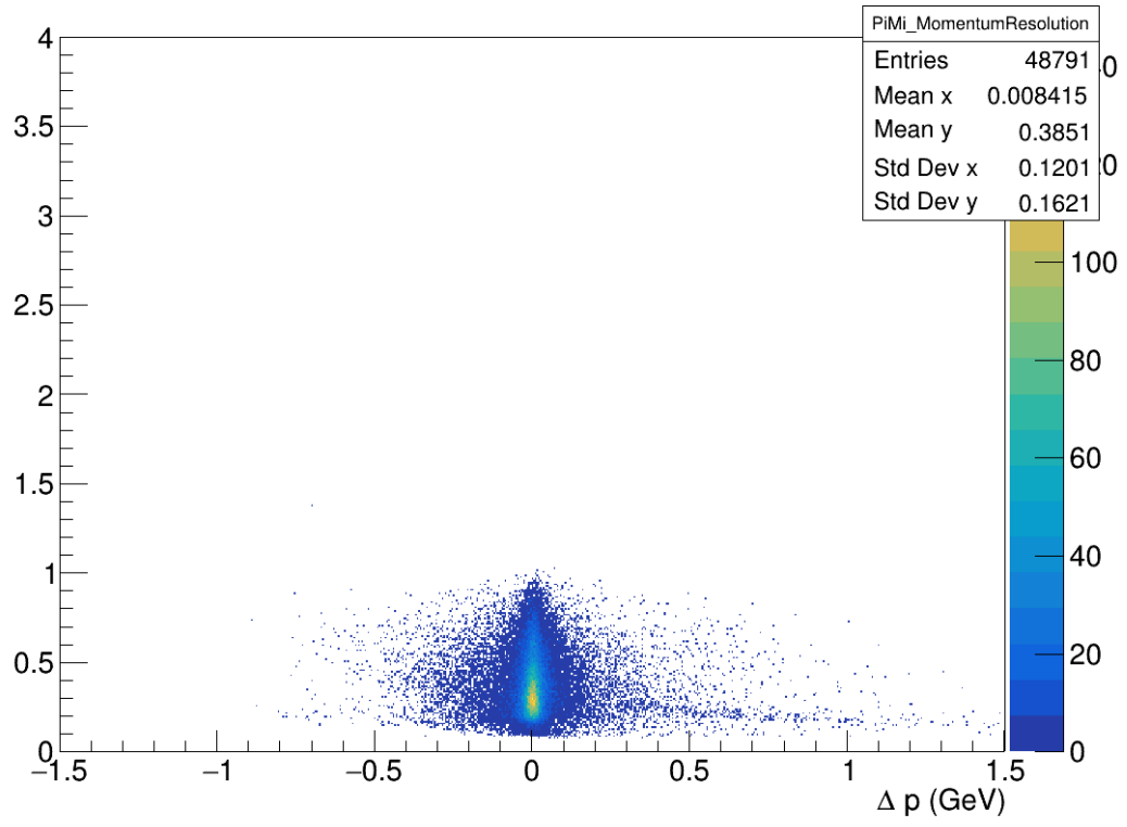
Figure 5: \pi^- Resolution
