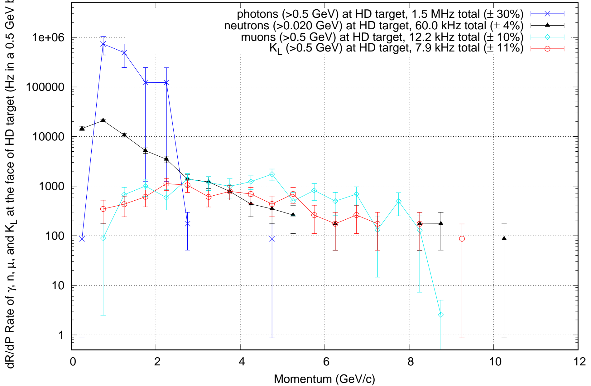
CPS 12 GeV, 5 \mu A on 10% R.L. radiator photon beam + KPT \rightarrow \gamma, n, \mu, K_L at HD target
