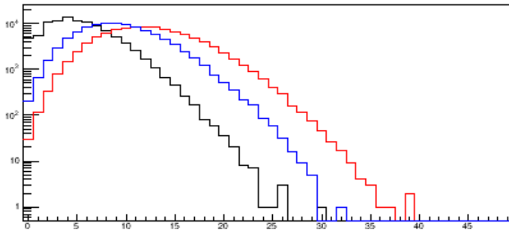
gamma multiplicity
