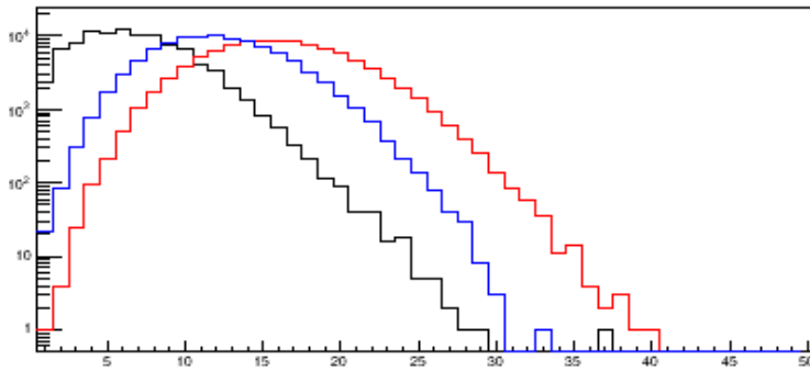
hadron multiplicity
