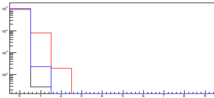
tau multiplicity
