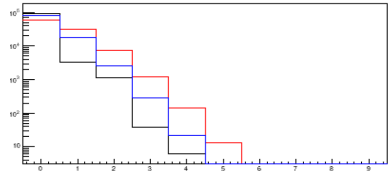
lepton multiplicity
