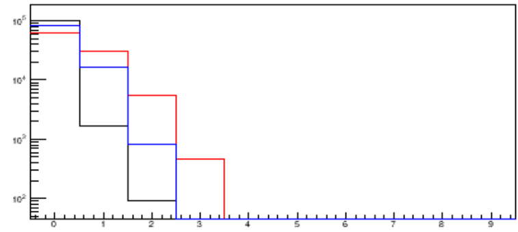
muon multiplicity
