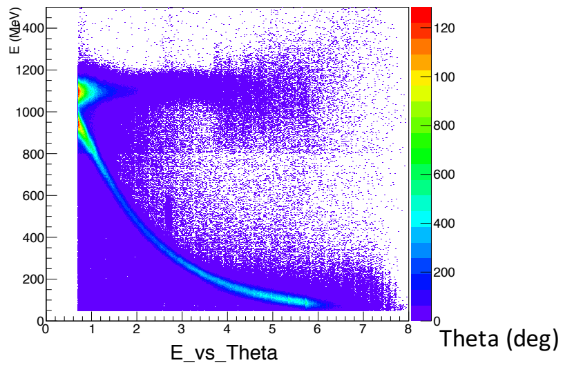
Cluster Energy E vs Scattering Angle \theta
