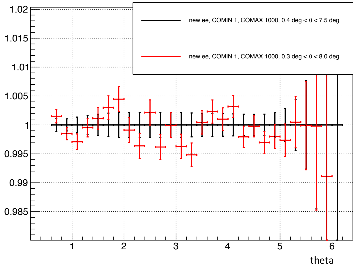
raw_yield_hist_s_ee1
