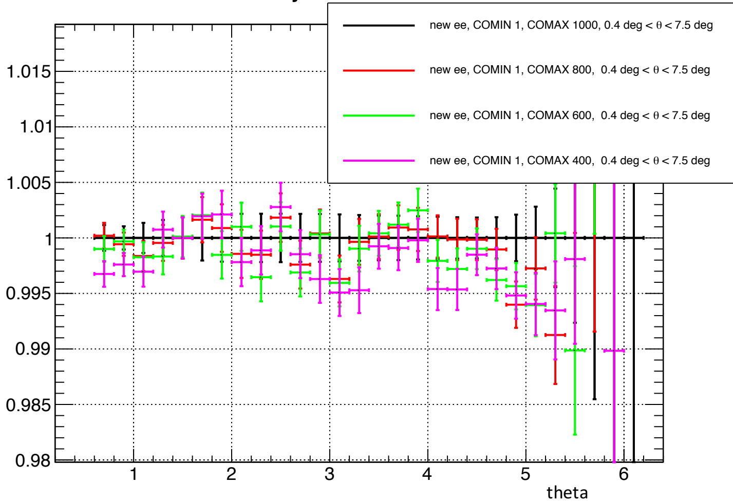
raw_yield_hist_s_ee1
