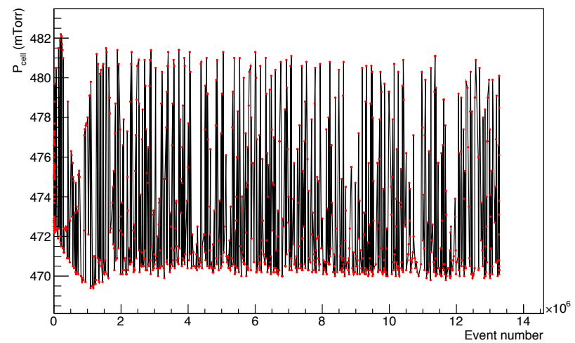
Cell_Pressure
