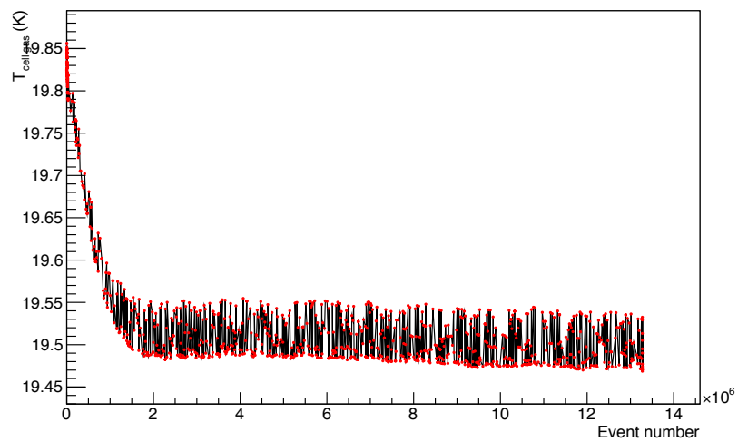
Cell_Gas_Temperature
