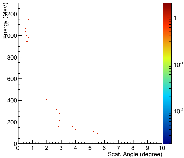
Reconstructed Hits
