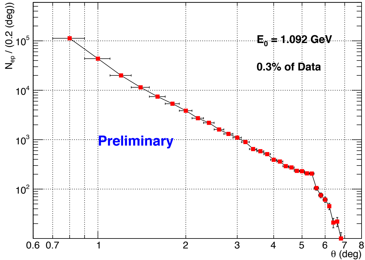
N_{ep \rightarrow ep} vs. Scattering Angle \theta
