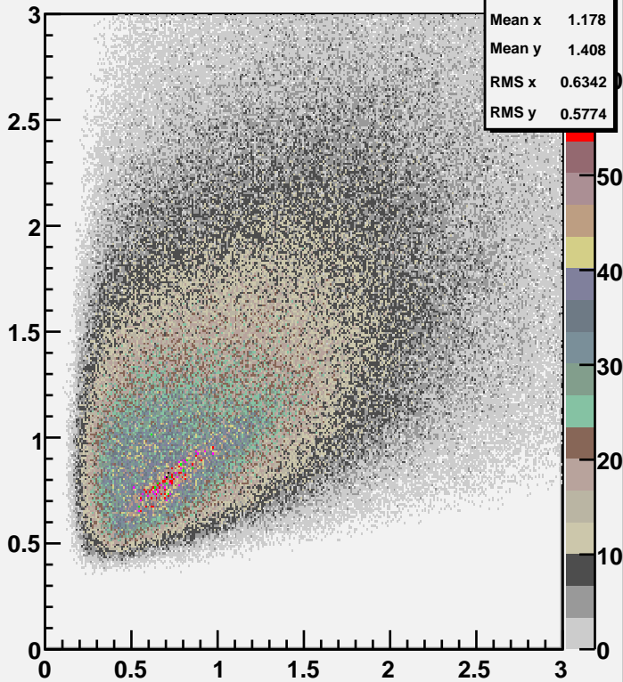
t(beam -> K-) vs t(gam -> K+K-) Plot 3
