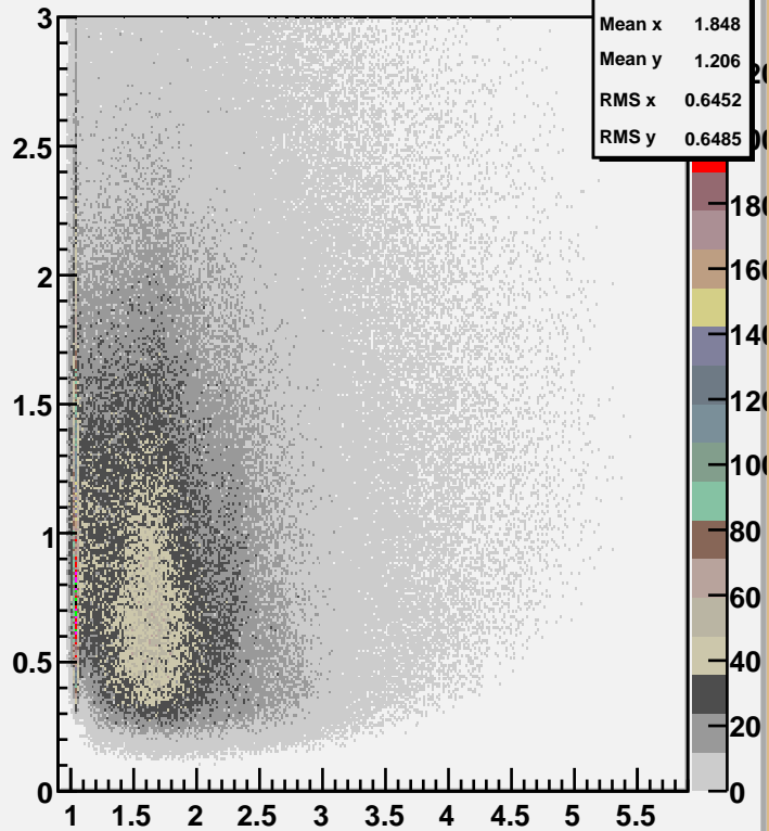
t(beam -> K+K-) vs m2(K+K-) Plot 4
