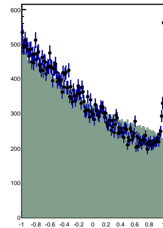
cos(Theta_u)
