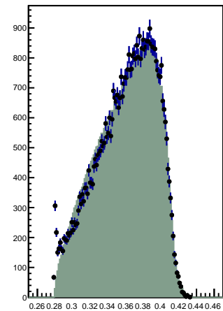
Mass( PI+ PI- )
