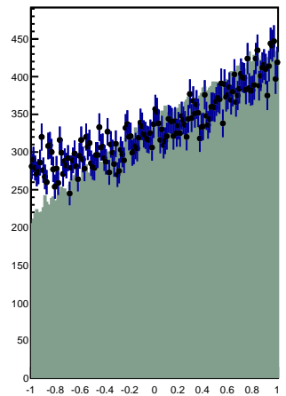
cos(Theta_s)
