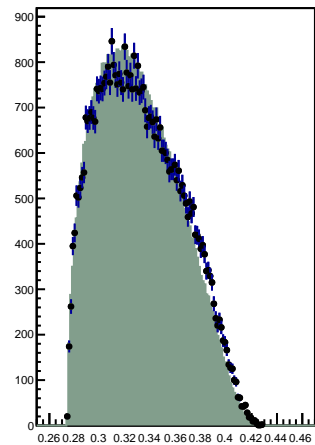
Mass( PI0 PI+ )
