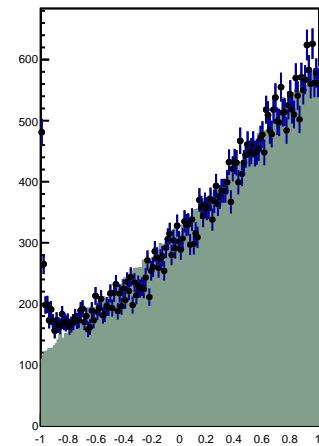
cos(Theta_t)
