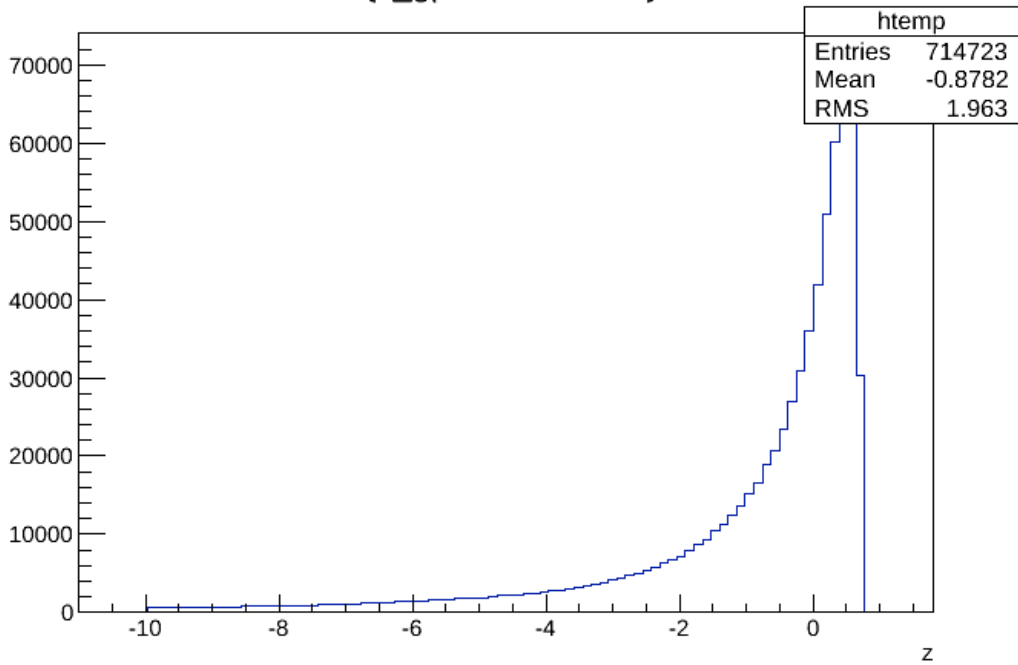
z {s_gp&gt;9.4&amp;&amp;z&gt;-10}
