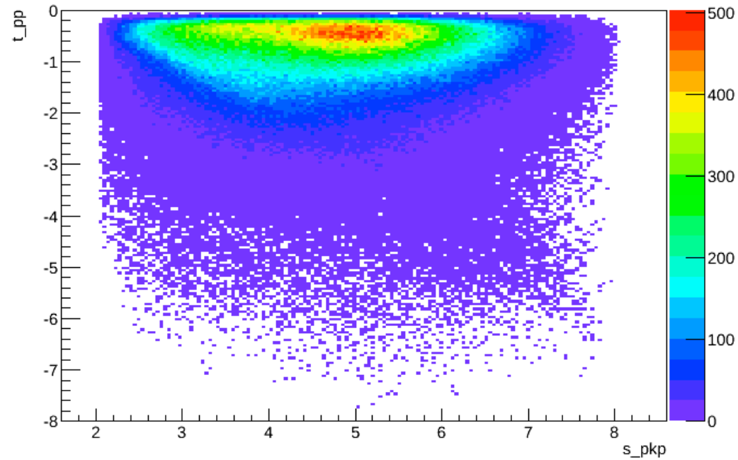
t_pp:s_pkp {s_gp>9.4}
