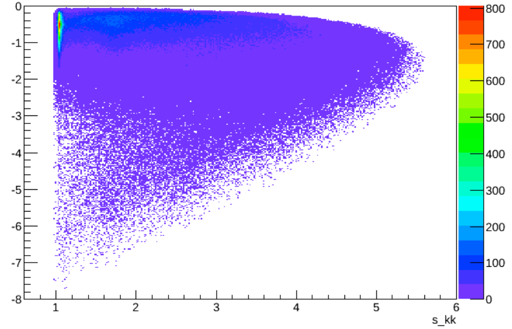
t_pp:s_kk {s_gp>9.4}
