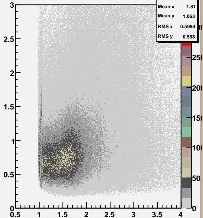
tK+ vs m2(K- K+) Plot 2
