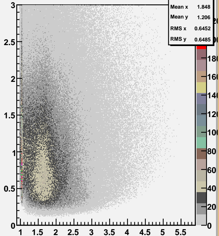
t(bean -&gt; K+K-) vs m2(K+K-) Plot 4
