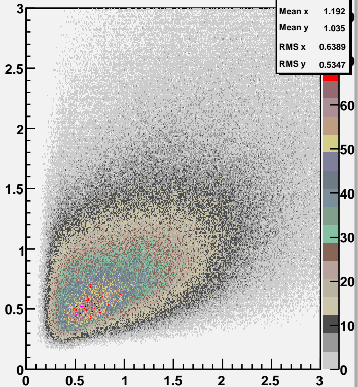
t(bean -&gt; K+) vs t(gam -&gt; K+K-) Plot 3
