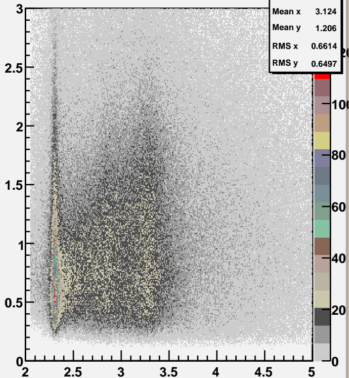
tK+K- vs m2(K- p) Plot 1
