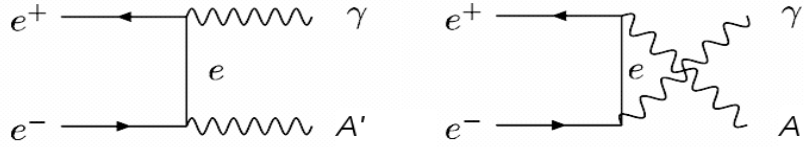
Figure 49. A' production via e^+e^- annihilation.
