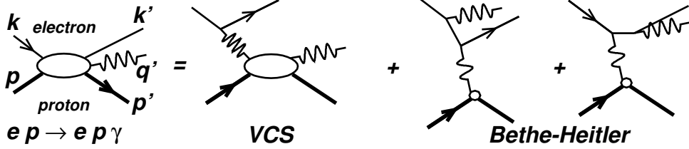
Figure 43. Lowest order QED amplitude for the ep \rightarrow ep\gamma reaction. The momentum four-vectors of all external particles are labeled at left. The net four-momentum transfer to the proton is \Delta_\mu = (q - q')_\mu = (p' - p)_\mu . In the virtual Compton scattering (VCS) amplitude, the (spacelike) virtuality of the incident photon is Q^2 = -q^2 = -(k - k')^2 . In the Bethe-Heitler (BH) amplitude, the virtuality of the incident photon is -\Delta^2 = -t . Standard (e, e') invariants are s_e = (k + p)^2 , x_B = Q^2/(2q \cdot p) and W^2 = (q + p)^2 .
