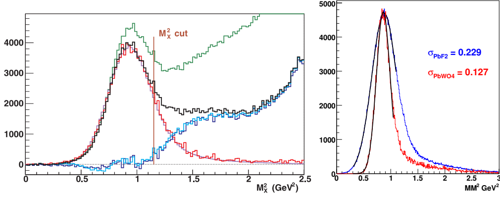
Figure 34. Left: Missing mass squared in E00-110 for H(e, e'\gamma)X events (green curve) at Q^2 = 2.3 \text{ GeV}^2 and -t \in [0.12, 0.4] \text{ GeV}^2 , integrated over the azimuthal angle of the photon \phi_{\gamma\gamma} . The black curve shows the data once the H(e, e'\gamma)\gamma X' events have been subtracted. The other curves are described in the text. Right: Projected missing mass resolution for a similar kinematic setting ( E_b = 6.6 \text{ GeV} , Q^2 = 3 \text{ GeV}^2 , x_B = 0.36 ). By using \text{PbWO}_4 instead of \text{PbF}_2 , the missing mass resolution will be considerably improved. Values are given in Tab. 7 and are to be compared to the value \sigma(M_X^2) = 0.2 \text{ GeV}^2 obtained in previous experiments in Hall A and showed in this figure (Left).
