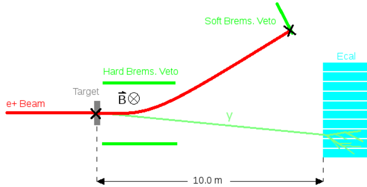
Figure 39. Schematic of the proposed experiment at Jefferson Lab.
