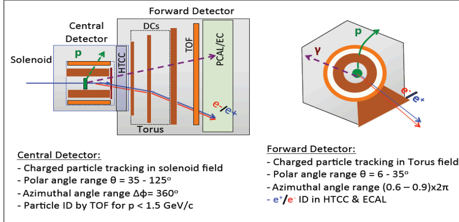
Figure 21. Generic CLAS12 configuration for the electron-proton and the positron-proton experiments. The central detector will detect the protons, and the bending in the magnetic solenoid field will be identical for the same kinematics. The electron and the positron, as well as the high-energy DVCS photon will be detected in the forward detector part. The electron and positron will be deflected in the torus magnetic field in the same way as the torus field direction will be opposite in the two experiments. The deflection in \phi due to the solenoid fringe field will be of same magnitude \Delta\phi but opposite in direction. The systematic of this shift can be controlled by doing the same experiment with opposite solenoid field directions that would result in the sign change of the \Delta\phi .
