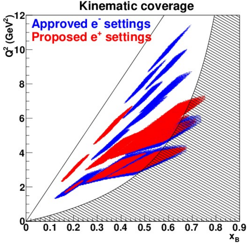
Figure 35. Display of different kinematic setting proposed. Blue corresponds the settings already approved in Hall A and Hall C using an electron beam. Red shows the proposed kinematics with positrons. Shaded areas show the resonance region W < 2 \text{ GeV} and the line Q^2 = (2M_p E_b)x_B limits the physical region for a maximum beam energy E_b = 11 \text{ GeV} .
